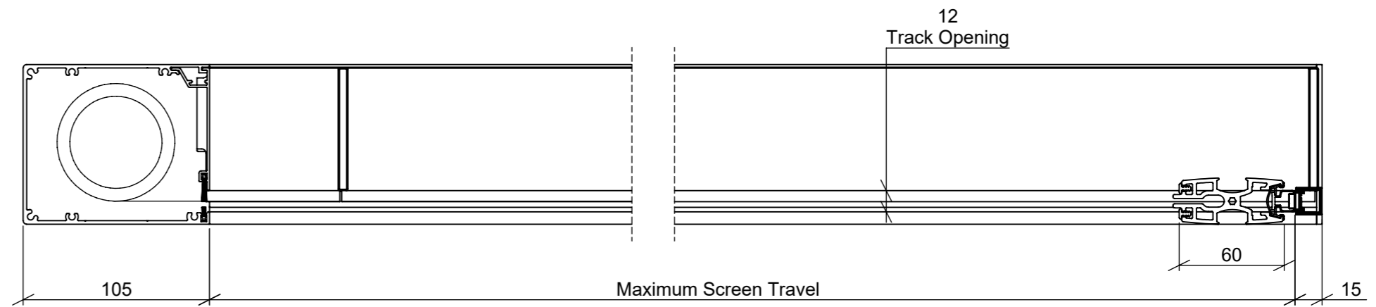
SECTION C-C
