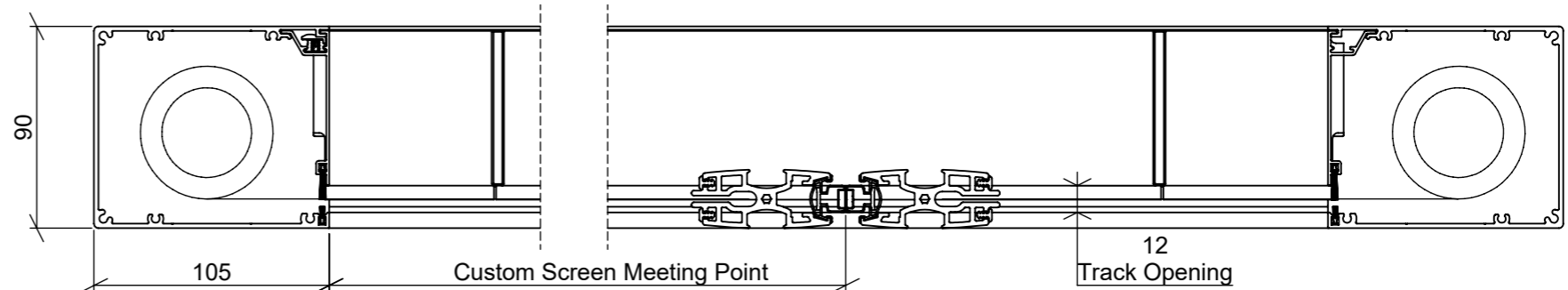
SECTION B-B
